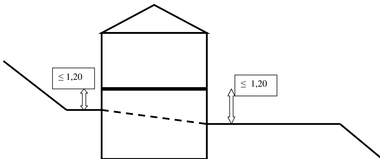
Figura 3 – PIANO INTERRATO Art. 2 comma 15
