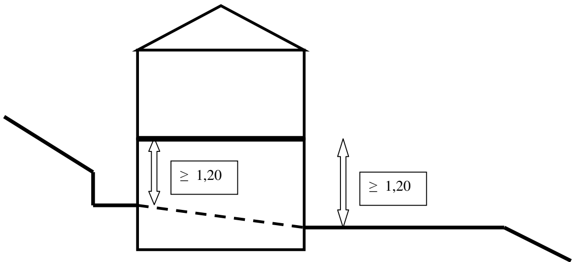
Figura 2 – PIANO SEMINTERRATO Art. 2 comma 14
